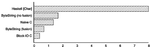
Fig. 1. Relative running times (seconds)
