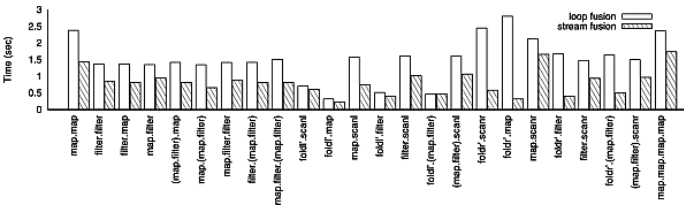
Fig. 3. Fusion strategies: loop versus stream fusion
