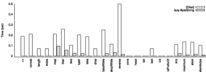
Fig. 2. [Char] and lazy ByteString : running time
