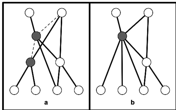
Fig. 2. Merge Mutation: (a) the gray nodes are about to be merged. The dashed lines indicate connections that will be deleted by the merge, and the solid lines are connections that will persist.
