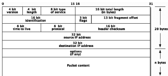
Figure 3. IP Header
