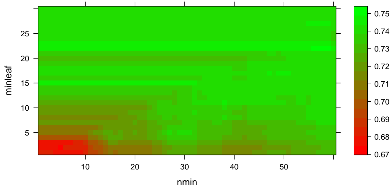
Success rate with Pima indians data set [%]
