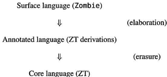
Figure 8. Implementation
